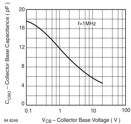
Figure 7. Collector Base Capacitance vs. Collector Base Voltage
