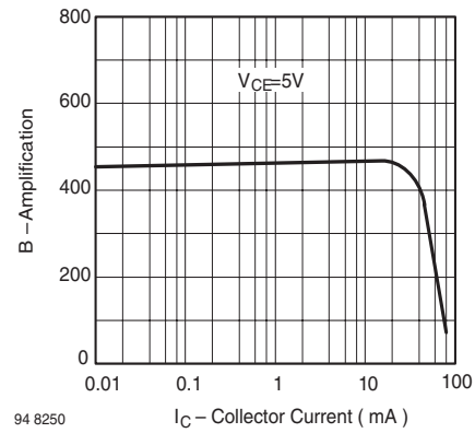
Figure 6. Amplification vs. Collector Current
