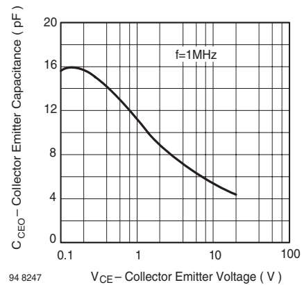
Figure 8. Collector Emitter Capacitance vs. Collector Emitter Voltage
