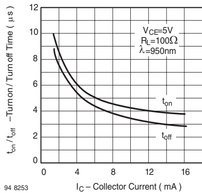
Figure 9. Turn On/Turn Off Time vs. Collector Current
