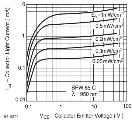
Figure 7. Collector Light Current vs. Collector Emitter Voltage
