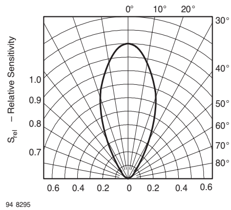
Figure 11. Relative Radiant Sensitivity vs. Angular Displacement
