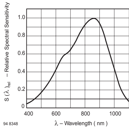
Figure 10. Relative Spectral Sensitivity vs. Wavelength
