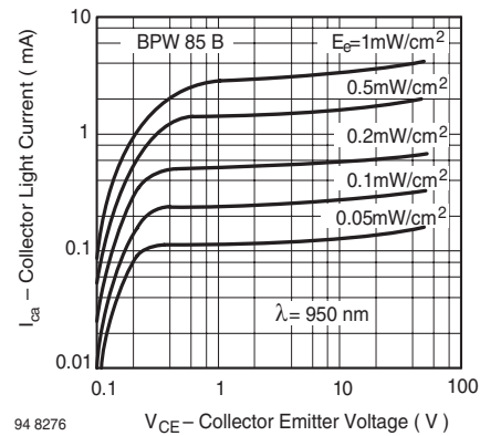
Figure 6. Collector Light Current vs. Collector Emitter Voltage
