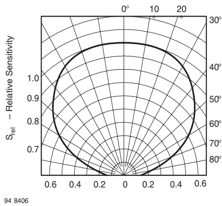
Figure 7. Relative Radiant Sensitivity vs. Angular Displacement
