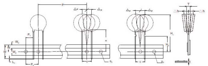
Figure 2 - PTR060V0250-PTR060V0375
