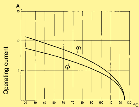
Ambient temperature
