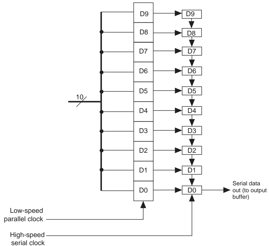
Figure 2-7. Serializer Note (1)
