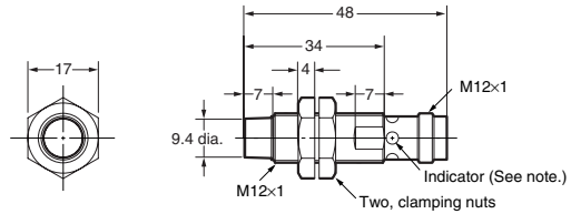
E2A-M12KN08-M1-□□/E2A-S12KN08-M1-□
