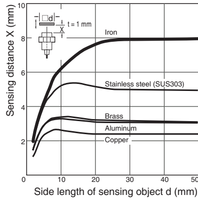
E2A-M12□N08/E2A-S12□N08
