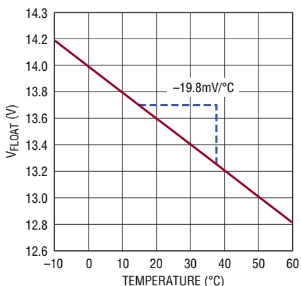
Figure 5. Lead-Acid 6-Cell Float Charge Voltage vs Temperature with a -19.8\text{mV}/^{\circ}\text{C} Temperature Coefficient Using LM234 with the Feedback Network
