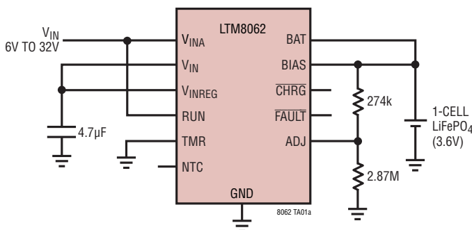
2A LiFePO 4 \mu Module Battery Charger
