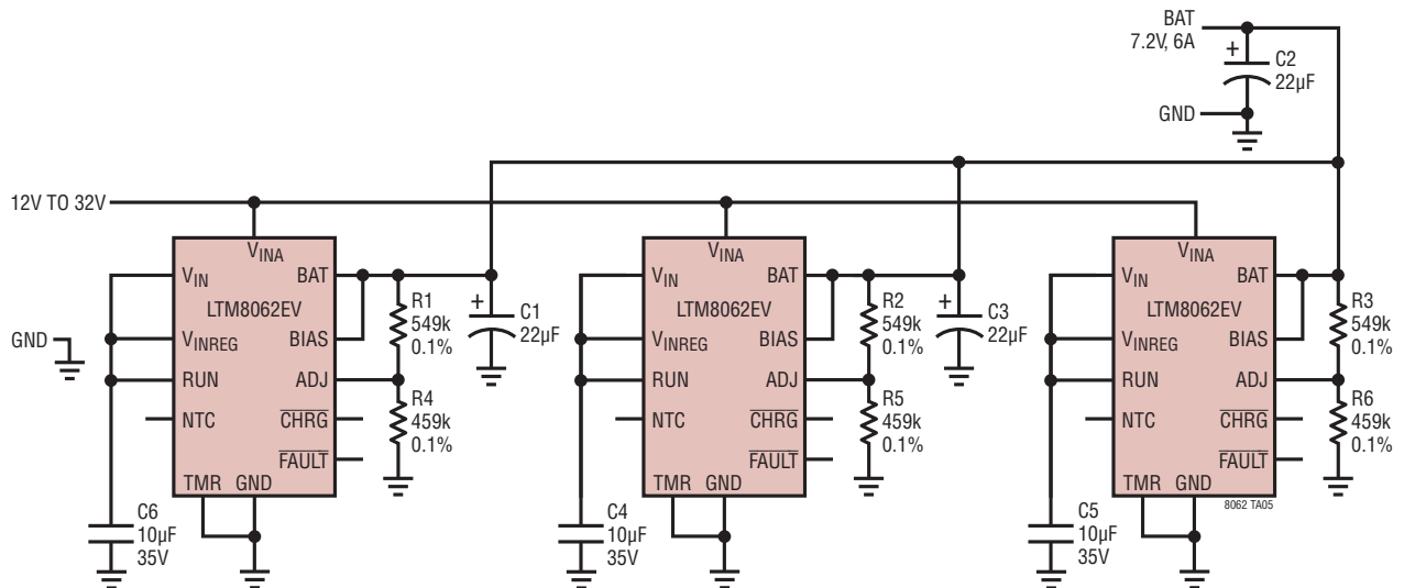
Two LTM8062s Operating In Parallel to Produce Higher Charge Current
