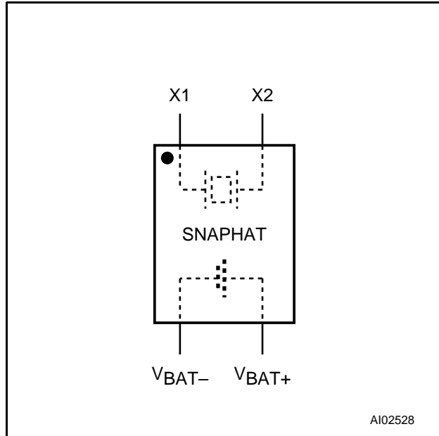
Figure 2. Logic Diagram
