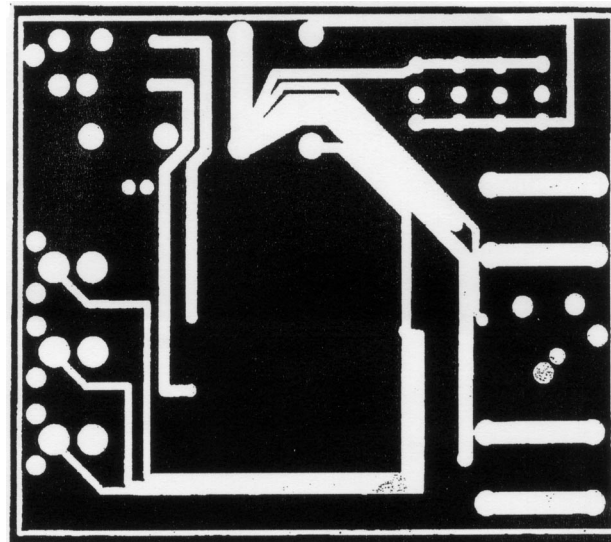
FIGURE 8. Inner Layer (3)
