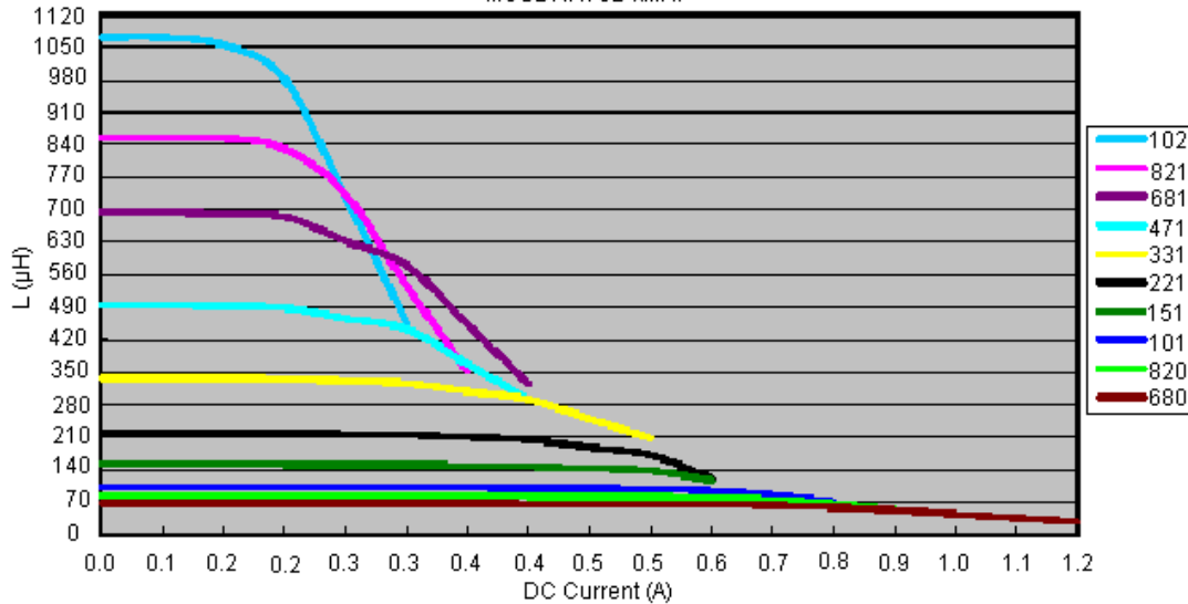
MCSDRH73B-xMHF
