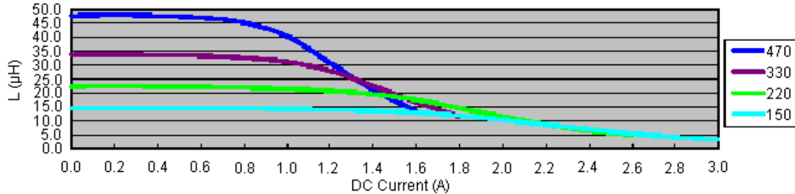
MCSDRH73B-xMHF
