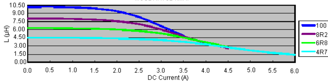
MCSDRH73B-xMHF
