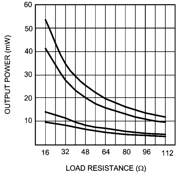
Output Power vs Load Resistance f = 1\text{kHz} , from top to bottom: V_{DD} = 3.0\text{V}, 10\%\text{THD+N}; V_{DD} = 3.0\text{V}, 1\%\text{THD+N} V_{DD} = 1.8\text{V}, 10\%\text{THD+N}; V_{DD} = 1.8\text{V}, 1\%\text{THD+N}
