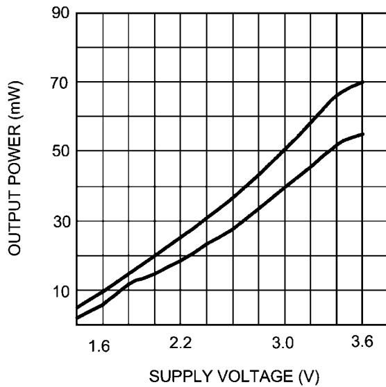
Output Power vs Supply Voltage R_L = 16\Omega , from top to bottom: \text{THD+N} = 10\%; \text{THD+N} = 1\%
