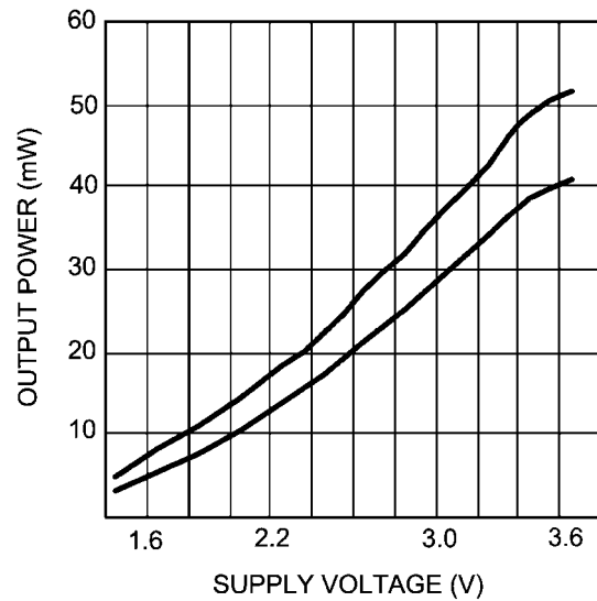
Output Power vs Supply Voltage R_L = 32\Omega , from top to bottom: \text{THD+N} = 10\%; \text{THD+N} = 1\%
