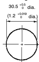
Mounting Holes
