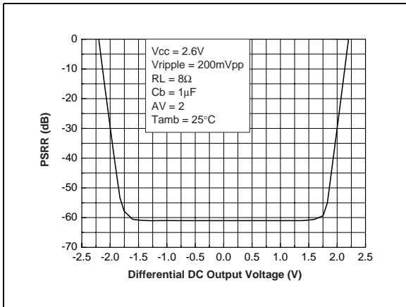
Figure 20. PSRR vs. DC output voltage
