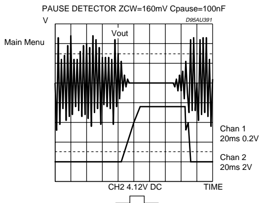
Figure 16: Pause Detector
