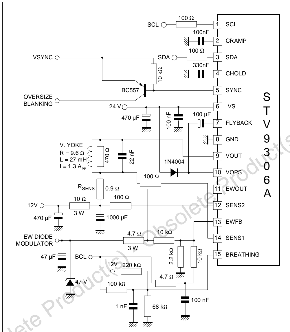
Figure 25: STV9306A Application Diagram
