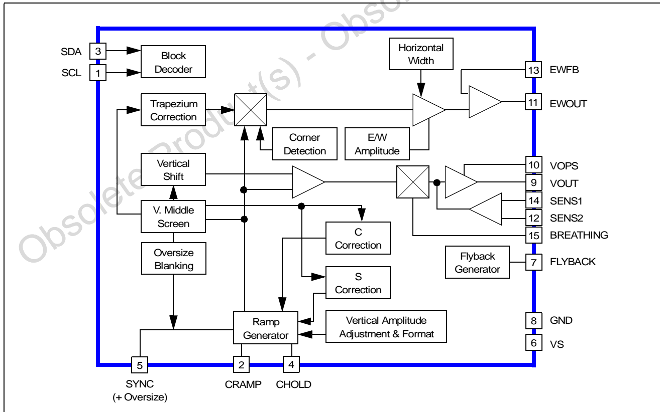
Figure 1: STV9306A Block Diagram
