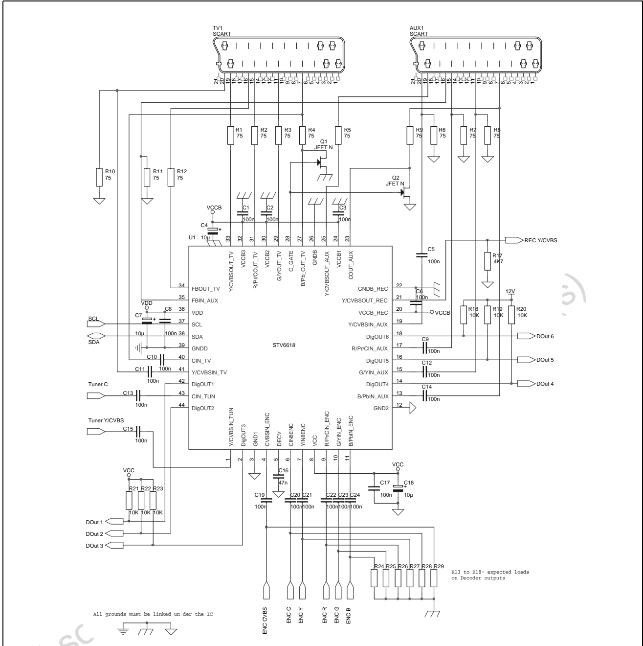
Figure 22: 2 SCART / RGB Signal Application
