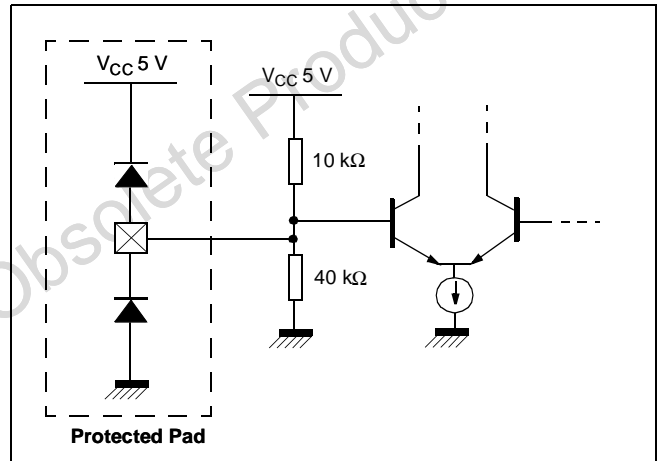
Figure 15: DECV (Pin 5)
