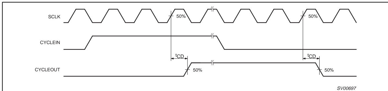
Figure 42. CYCLEOUT Waveforms
