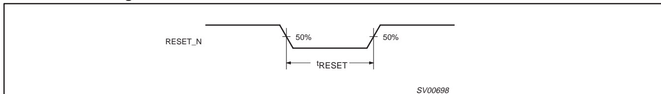
Figure 43. RESET_N Waveform
