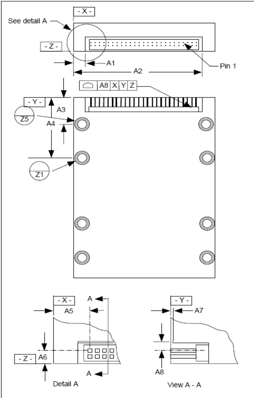
Figure 15: Connector location
