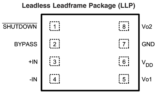
Top View Order Number LM4879SD See NS Package Number SDC08A
