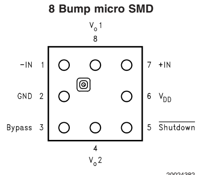
Top View Order Number LM4879IBP, LM4879IBPX See NS Package Number BPA08DDB
