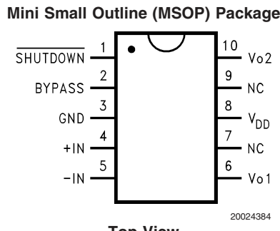
Top View NC = No Connect Order Number LM4879MM See NS Package Number MUB10A
