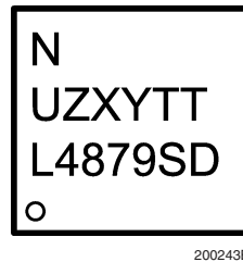
Top View N - NS Logo U - Fab Code Z - Assembly Plant Code XY - Date Code TT - Die Traceability L4879SD - LM4879SD
