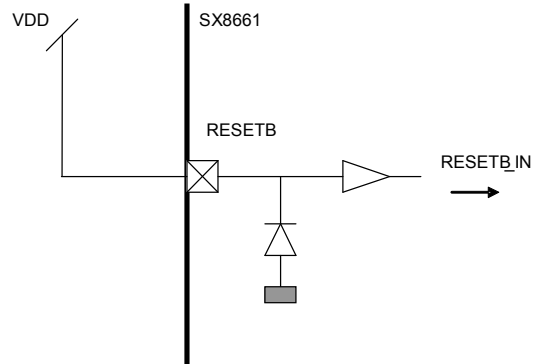
Figure 47 Simplified diagram of RESETB without host control
