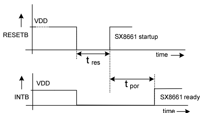
Figure 26 Hardware Reset
