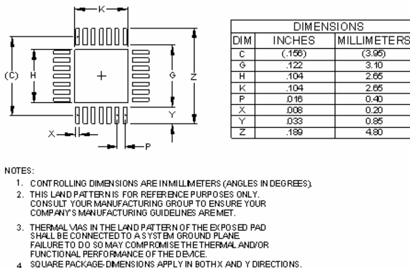
Figure 73 Land pattern
