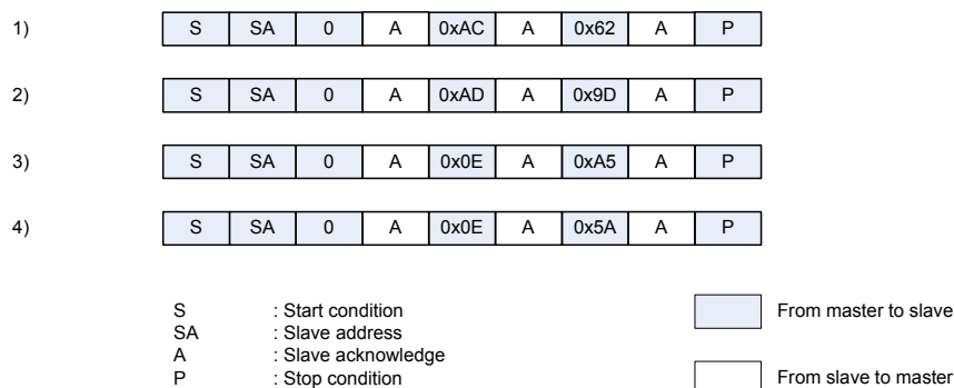
Figure 61: NVM burn procedure
