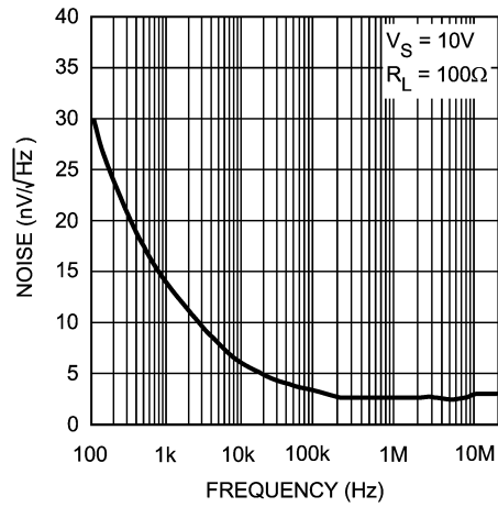
Voltage Noise
