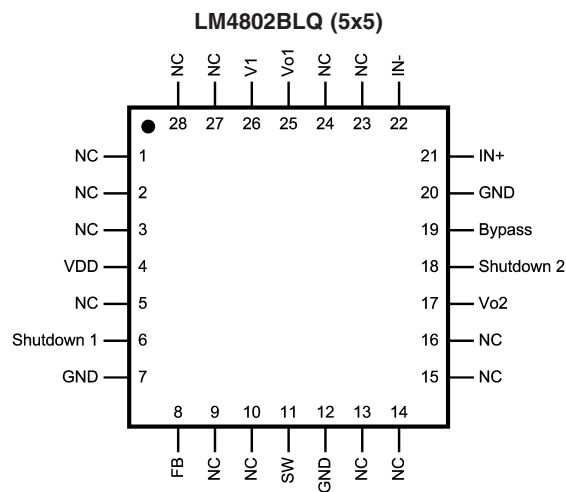
Top View Order Number LM4802BLQ See NS Package Number 2LQAQ028
