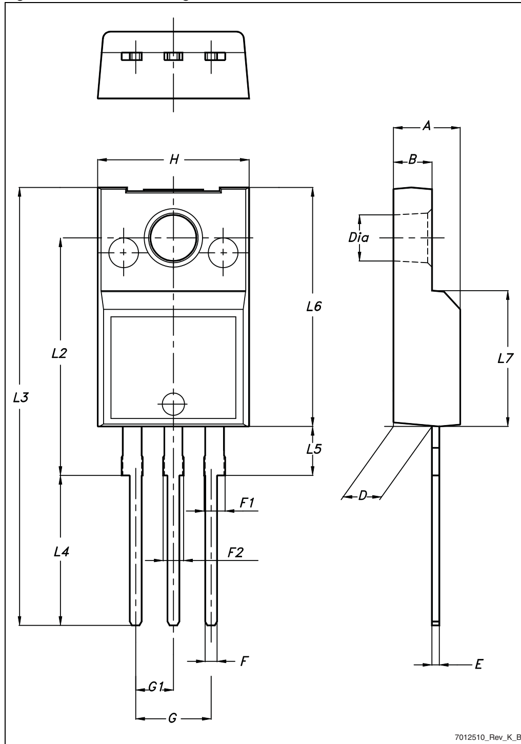
Figure 25. TO-220FP drawing
