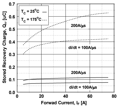
Figure 23. Stored Charge
