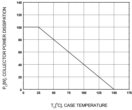
Figure 7. Power Derating
