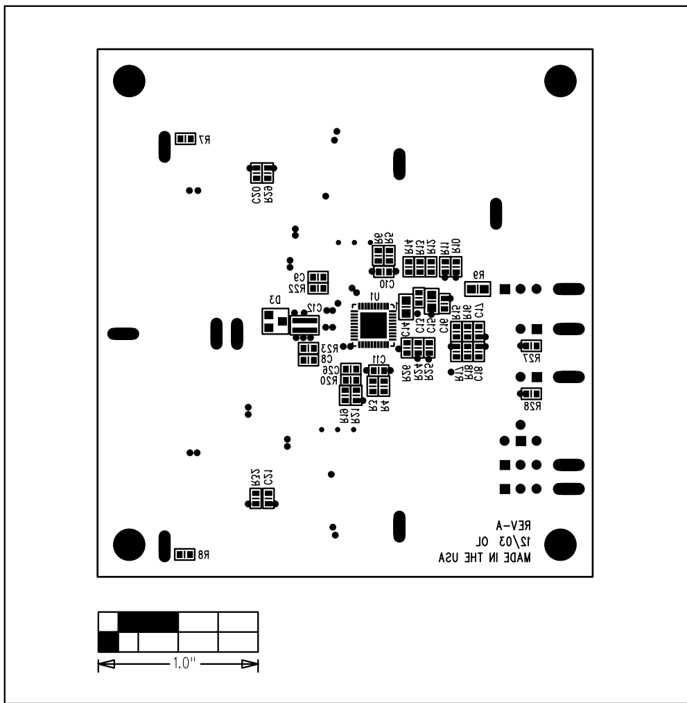
Figure 3. MAX1549 EV Kit Component Placement Guide—Solder Side
