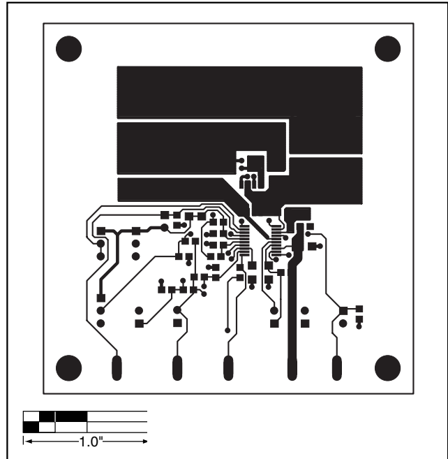
Figure 3. MAX1844 EV Kit PC Board Layout—Component Side
