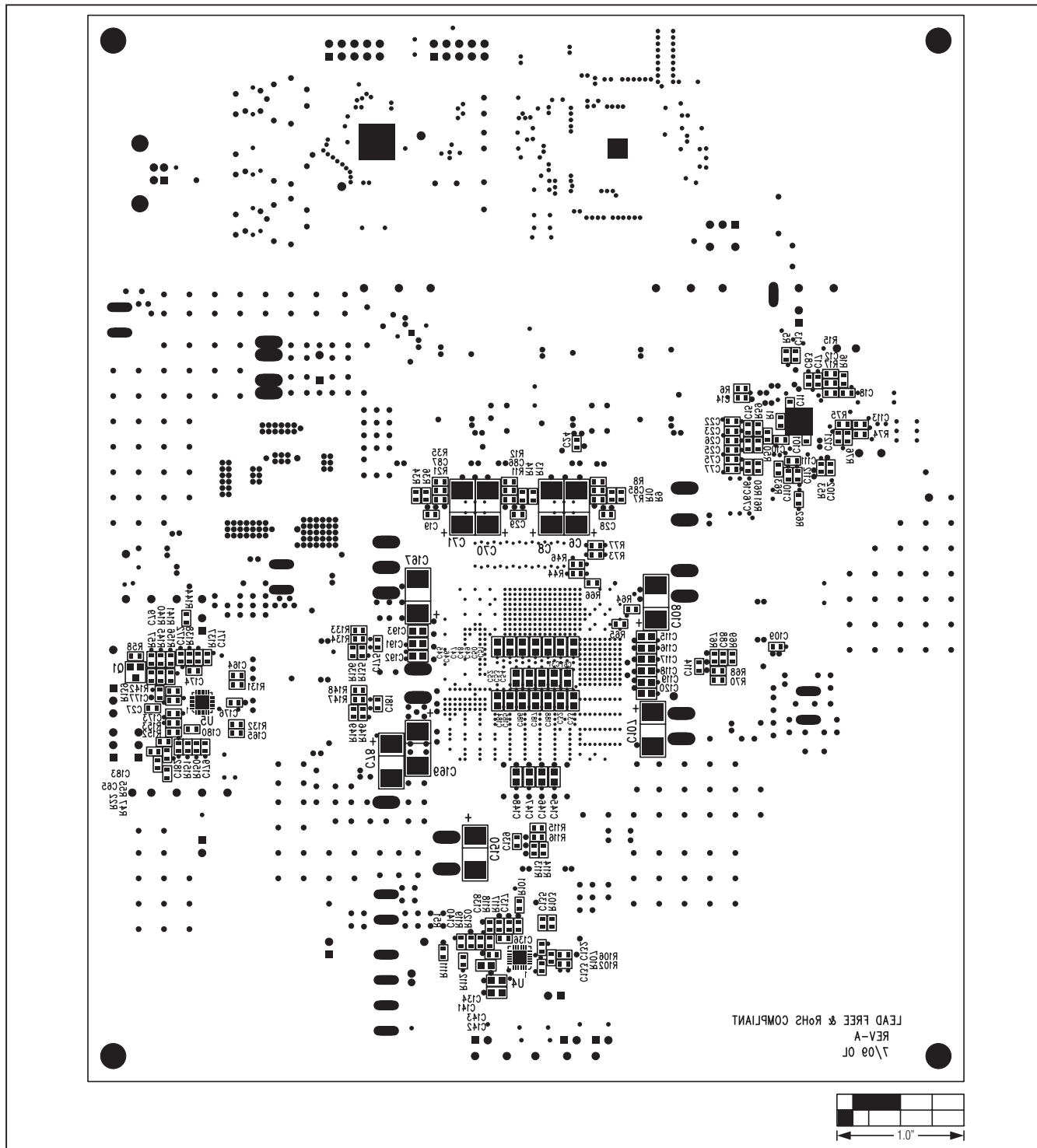
Figure 15. MAX17039 EV Kit Component Placement Guide—Solder Side
