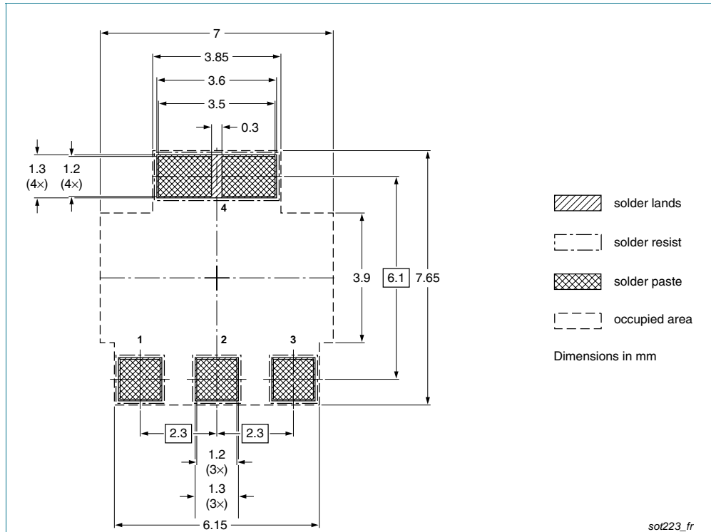
Fig 16. Reflow soldering footprint
