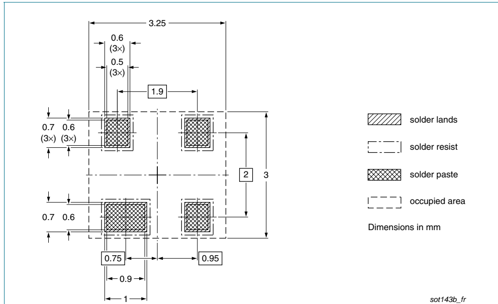
Fig 10. Reflow soldering footprint SOT143B
