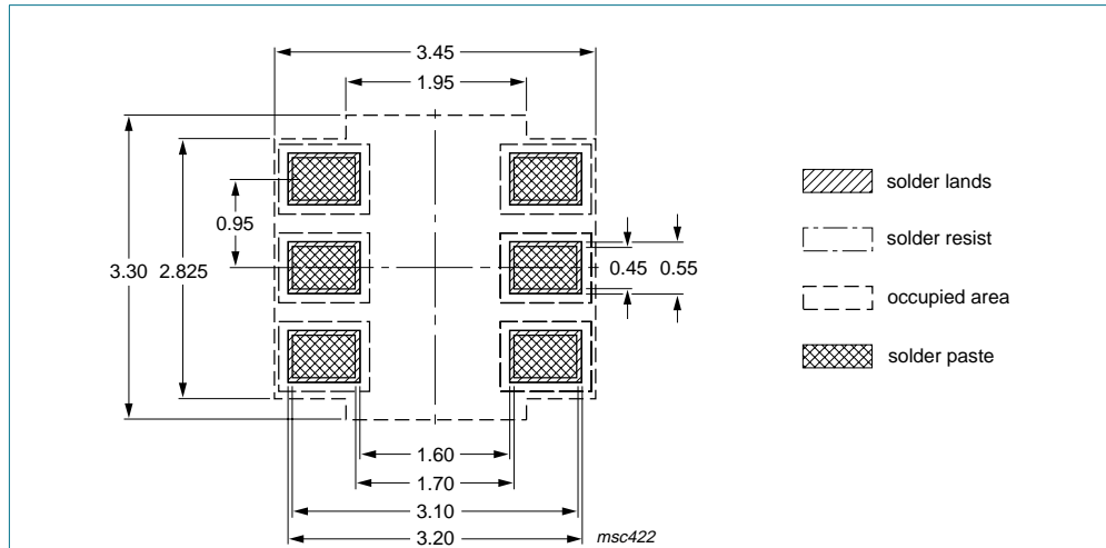
Fig 17. Reflow soldering footprint SOT457 (SC-74)
