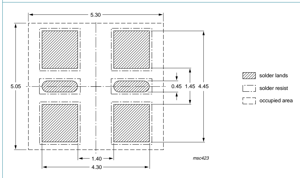
Fig 16. Reflow soldering footprint SOT457 (SC-74)
