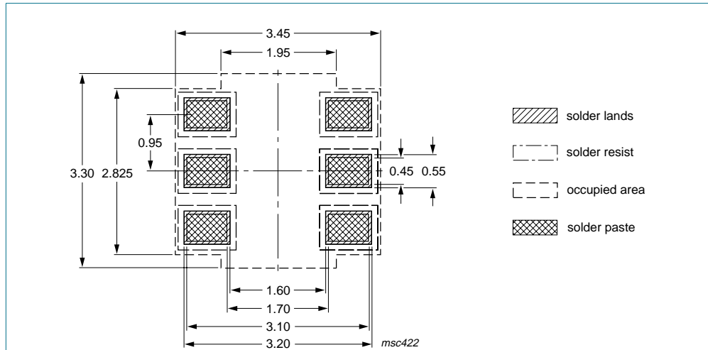
Fig 16. Reflow soldering footprint SOT457 (SC-74)
