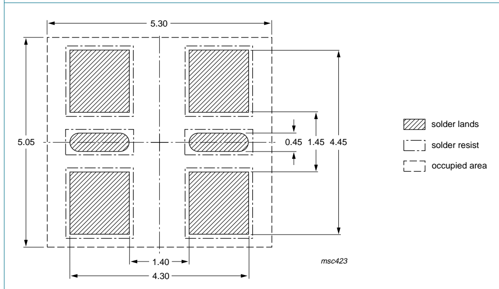
Fig 16. Reflow soldering footprint SOT457 (SC-74)
