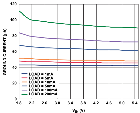
Figure 16. Ground Current vs. Input Voltage, Single Output Loaded
