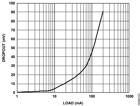
Figure 24. Dropout Voltage vs. Load Current and Output Voltage, V_{OUT1} = 3.3 V
