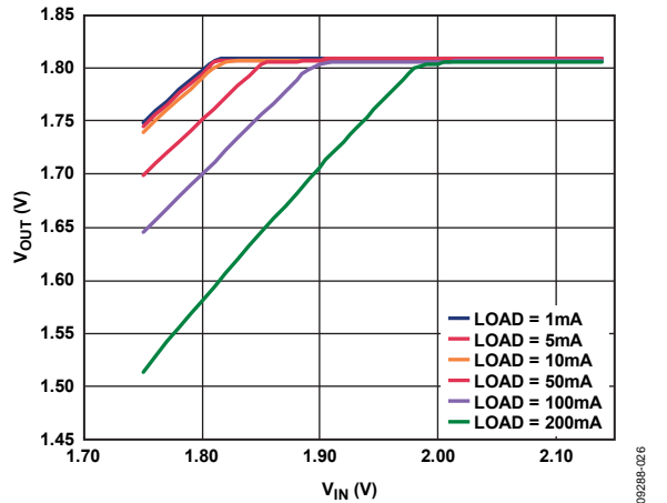
Figure 28. Output Voltage vs. Input Voltage (in Dropout), V_{OUT2} = 1.8 V
