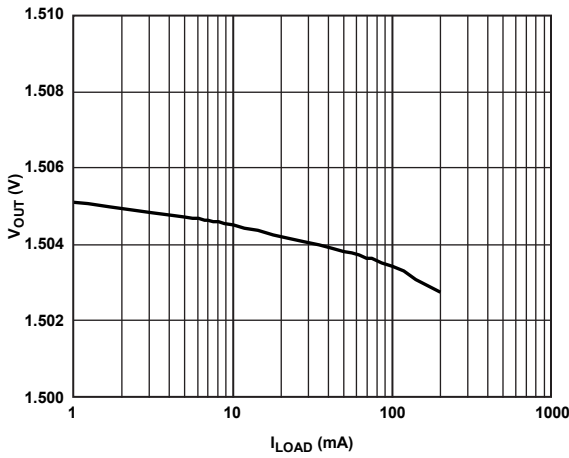
Figure 12. Output Voltage vs. Load Current
