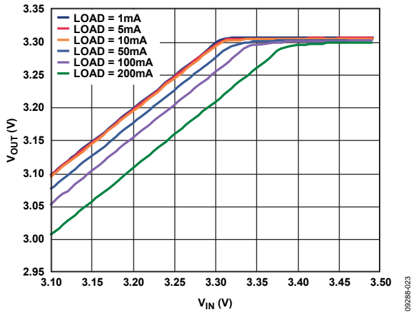
Figure 25. Output Voltage vs. Input Voltage (in Dropout), V_{OUT1} = 3.3 V
