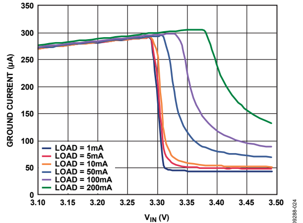
Figure 26. Ground Current vs. Input Voltage (in Dropout), V_{OUT1} = 3.3 V
