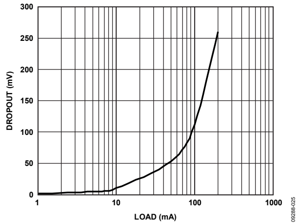
Figure 27. Dropout Voltage vs. Load Current and Output Voltage, V_{OUT2} = 1.8 V
