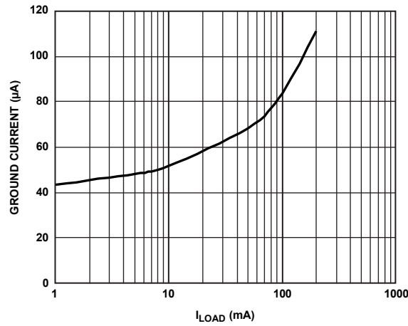
Figure 15. Ground Current vs. Load Current, Single Output Loaded
