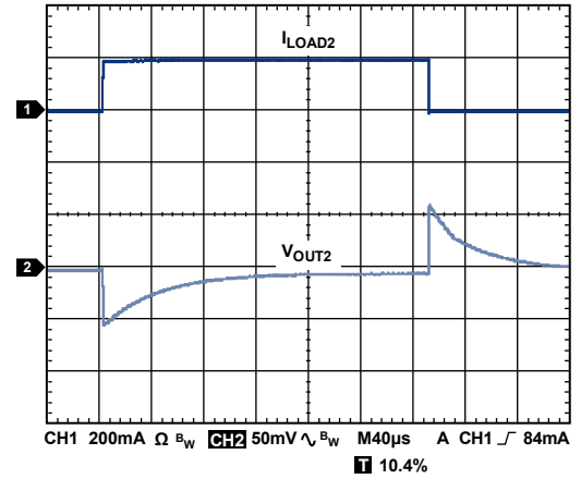
Figure 38. Load Transient Response, I_{LOAD2} = 1\text{ mA to } 200\text{ mA} , C_{OUT2} = 1\text{ }\mu\text{F} , CH1 = I_{LOAD2} , CH2 = V_{OUT2}
