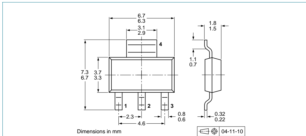
Fig 23. Package outline SOT223 (SC-73)
