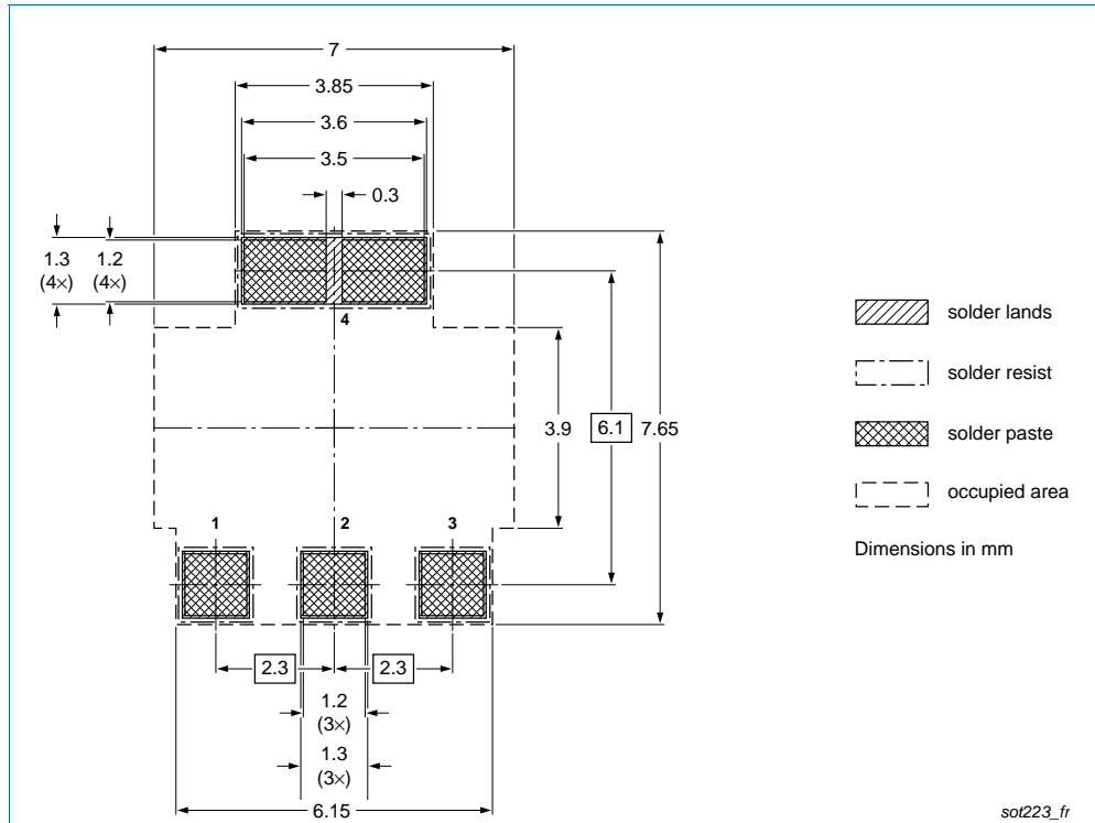
Fig 26. Reflow soldering footprint SOT223 (SC-73)
