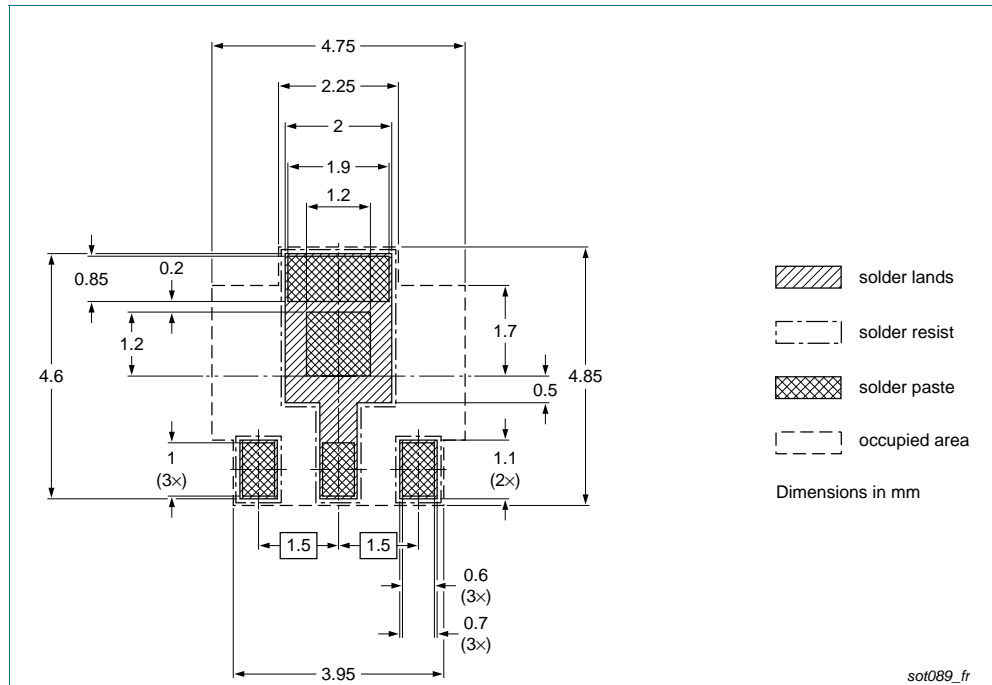
Fig 28. Reflow soldering footprint SOT89 (SC-62/TO-243)
