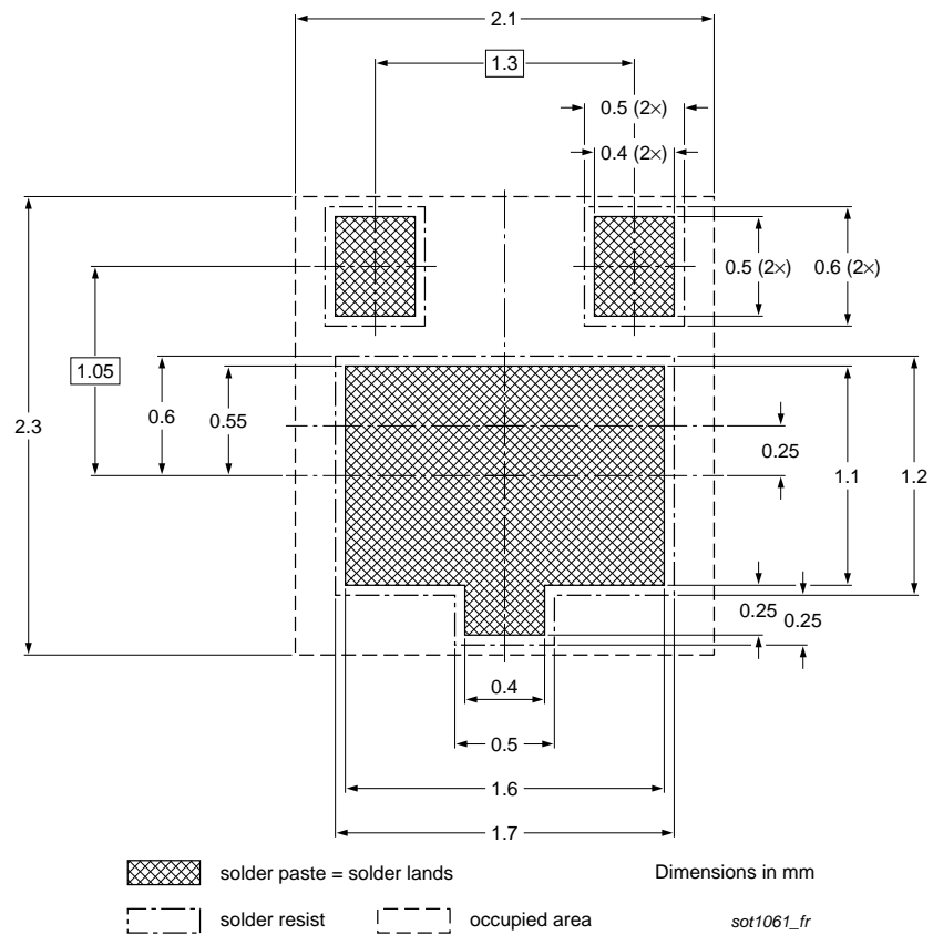
Fig 26. Reflow soldering footprint SOT1061 (HUSON3)
