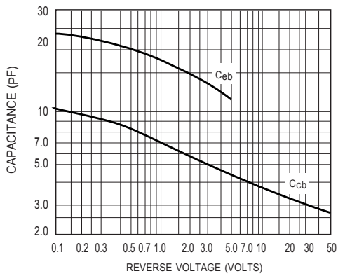
Figure 7.Capacitances
