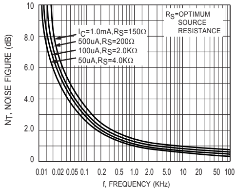
Figure 5.Frequency Effects
