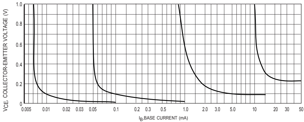
Figure 2. Collector Saturation Region
