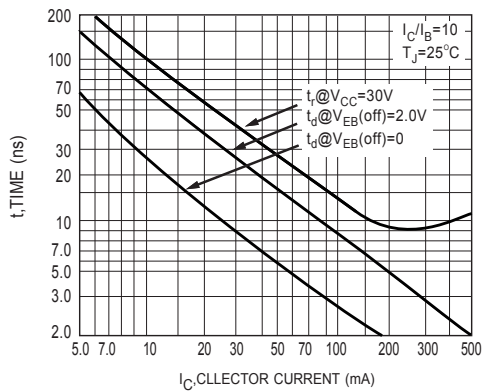
Figure 3. Turn-On Time
