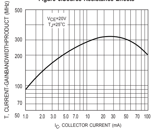
Figure 8.Currunt-Gain Bandwidth Product
