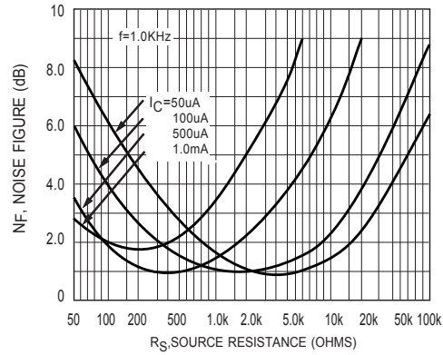
Figure 6.Source Resistance Effects
