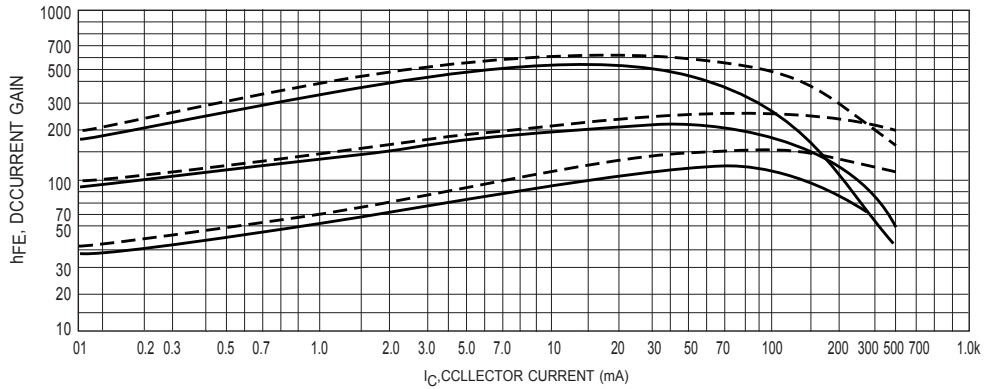
Figure 1. DC Current Gain
