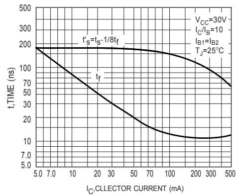
Figure 4. Turn-Off Time
