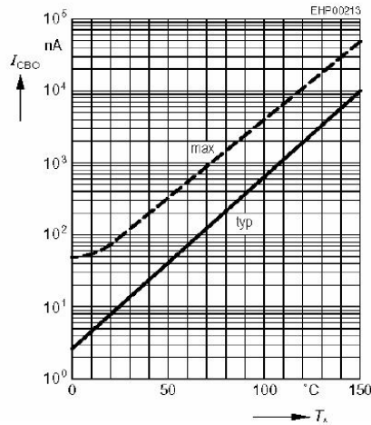
Collector cutoff current I_{CBO} = f(T_A) V_{CB} = 25V
