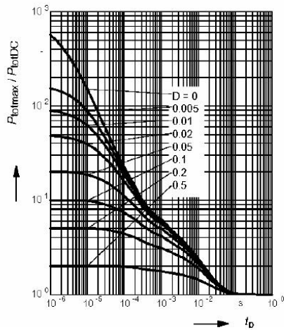
Permissible Pulse Load P_{totmax} / P_{totDC} = f(t_p)
