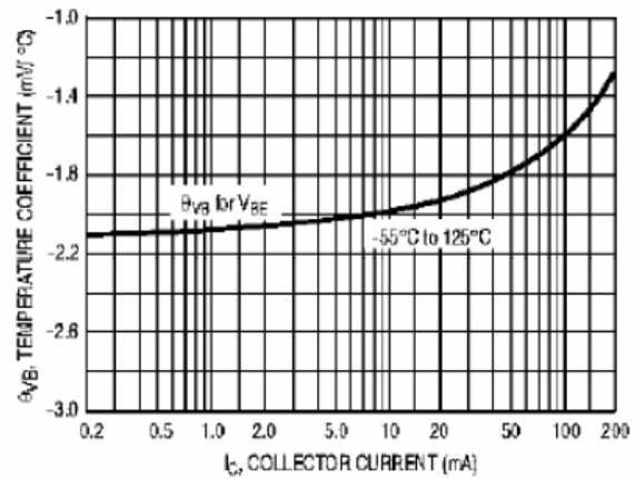
Figure 10. Base-Emitter Temperature Coefficient
