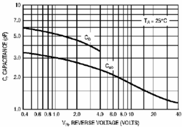
Figure 5. Capacitances
