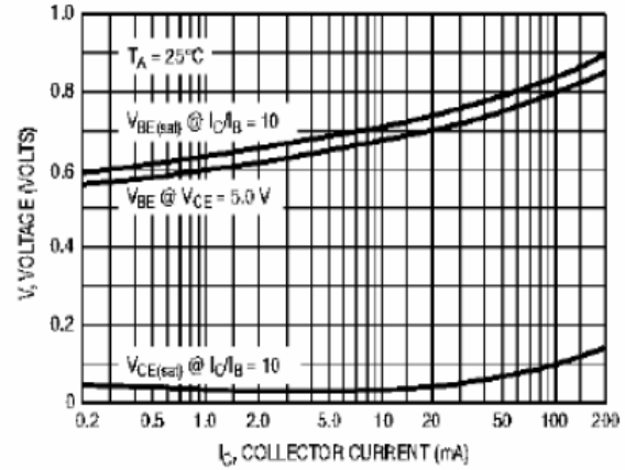
Figure 8. "On" Voltage
