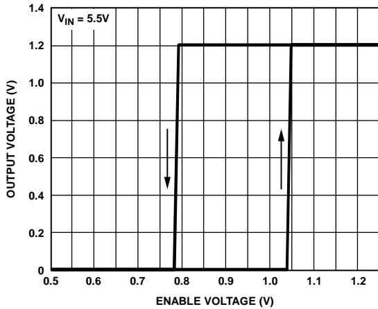
Figure 67. Typical ENx Pin Operation, VIN = 5.5 V
