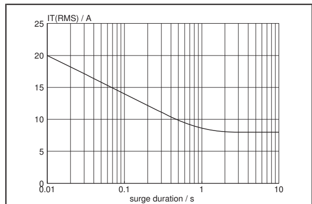
Fig.5. Maximum permissible repetitive rms on-state current I_{T(RMS)} , versus surge duration, for sinusoidal currents, f = 50 Hz; T_{hs} \leq 73^\circ C.
