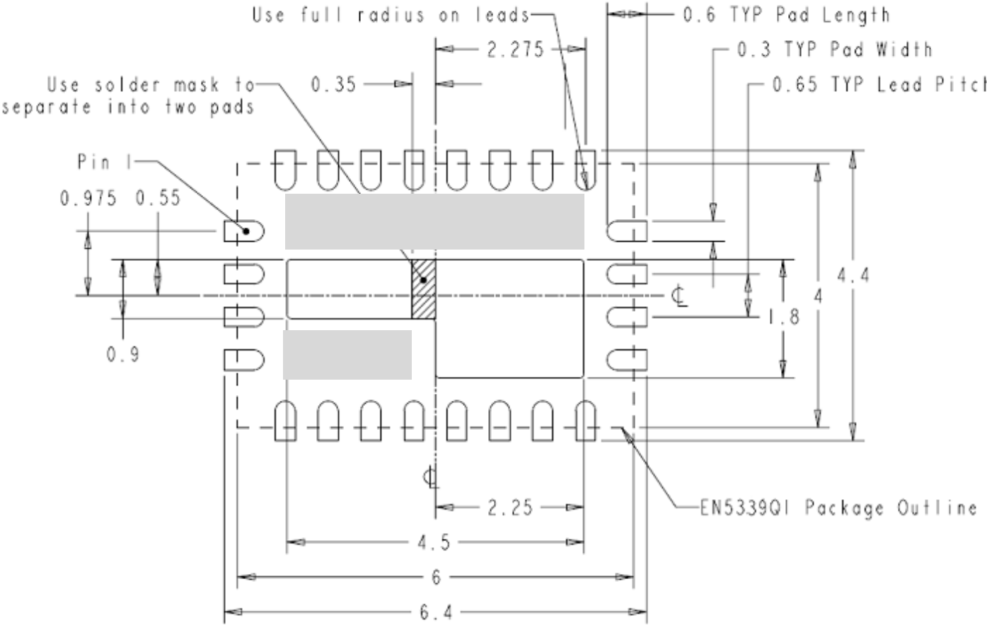
Figure 7. Recommended Footprint for PCB (Top View)
