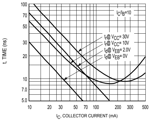
Figure 3. Turn-On Time
