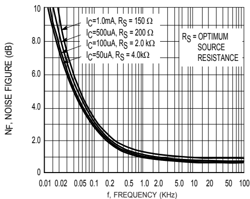
Figure 7. Frequency Effects
