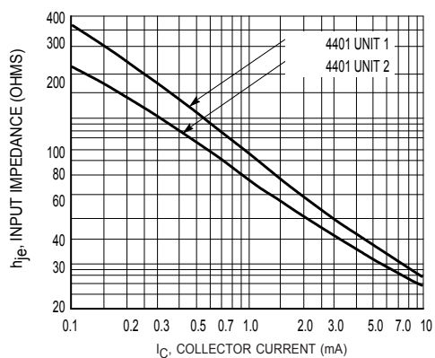
Figure 10. Input Impedance
