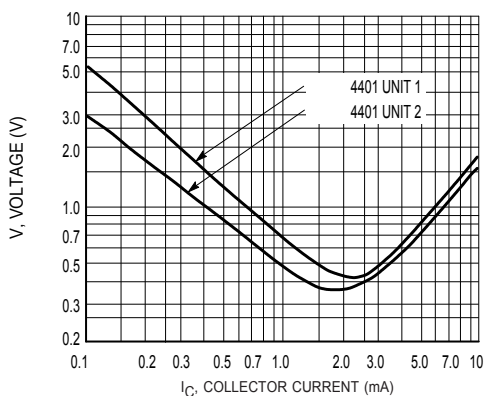
Figure 11. Voltage Feedback Ratio
