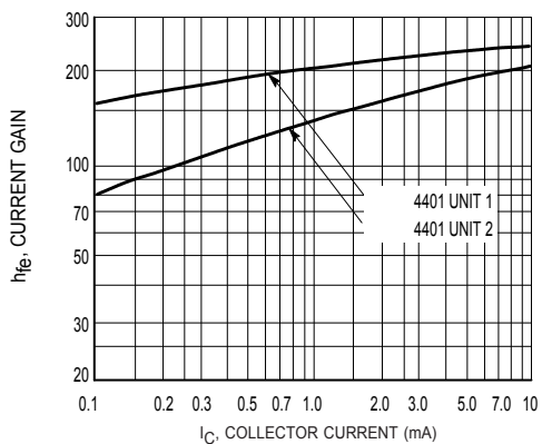
Figure 9. Current Gain
