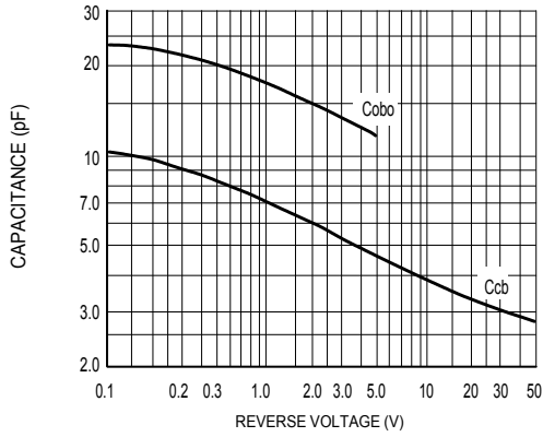
Figure 1. Capacitances
