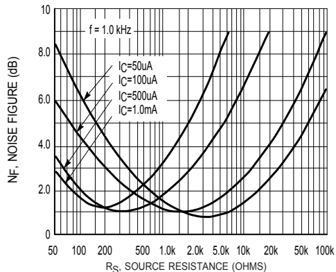
Figure 8. Source Resistance Effects
