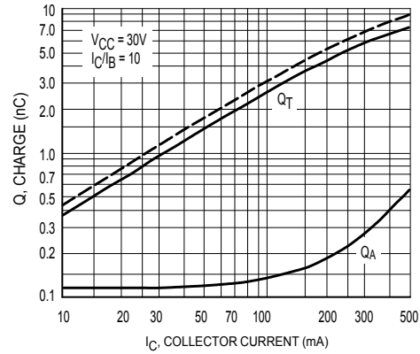
Figure 2. Charge Data
