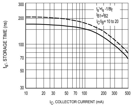
Figure 5. Storage Time
