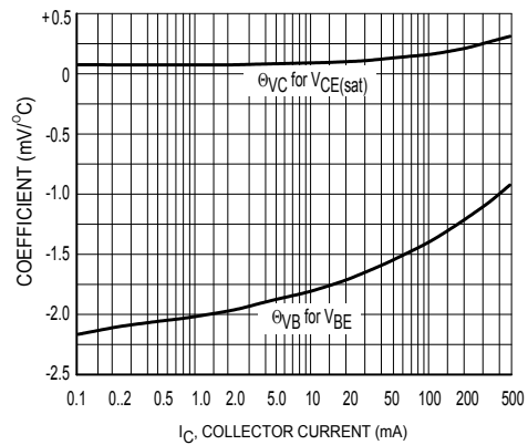
Figure 16. Temperature Coefficients
