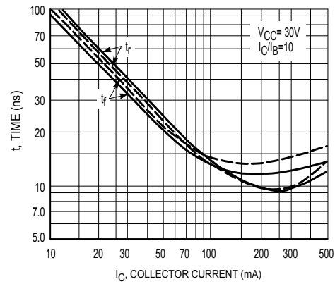
Figure 4. Rise and Fall Times
