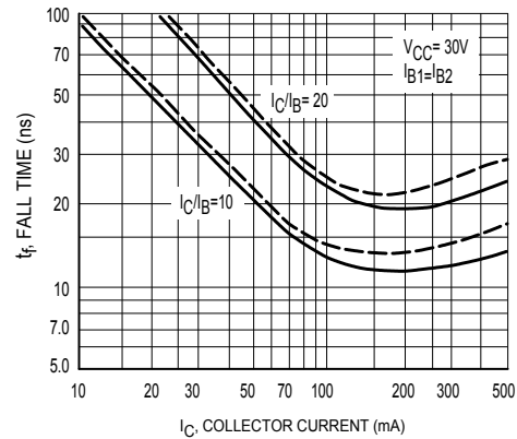
Figure 6. Fall Time
