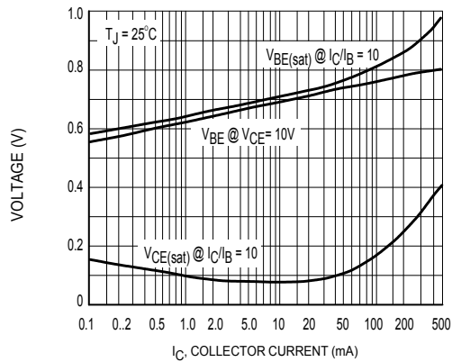
Figure 15. "ON" Voltages
