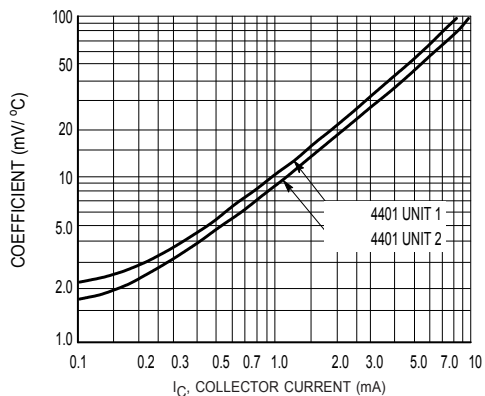
Figure 12. Temperature Coefficients
