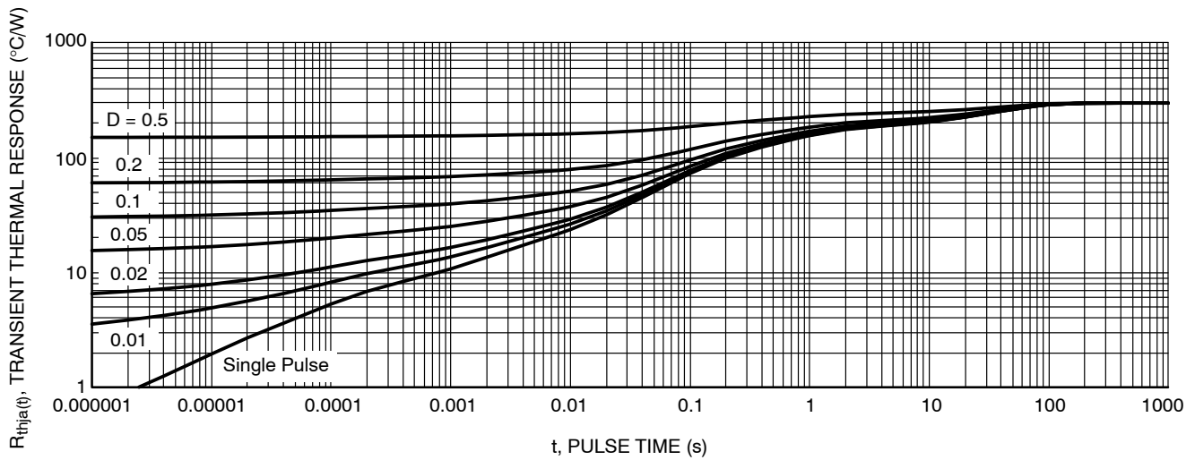
Figure 18. Thermal Response
