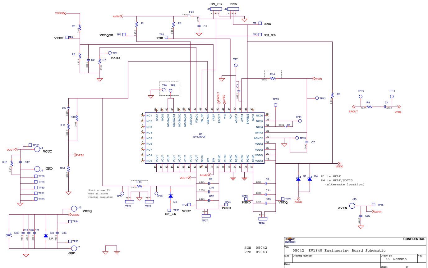
Figure 5: Evaluation Board Schematic
