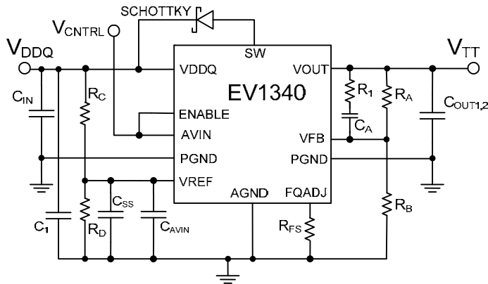
Figure 1: Output voltage programming and loop compensation
