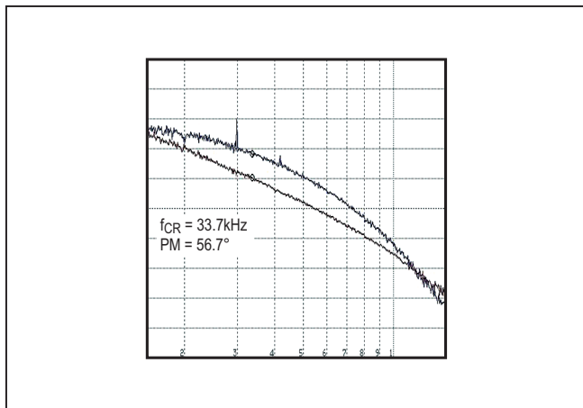
Figure 3. MAX17502H Full Load Bode Plot ( V_{IN} = 24V )
