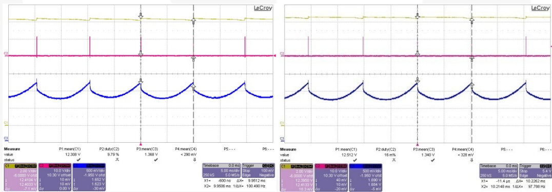
Figure 7. 90 V / 60 Hz at No Load, Ch1: V DD , Ch2: V GATE , Ch3: FB
