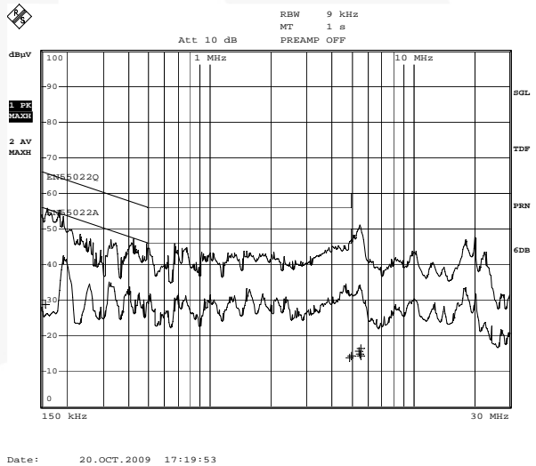
Figure 27. Conduction-Line & Neutral At 115V AC
