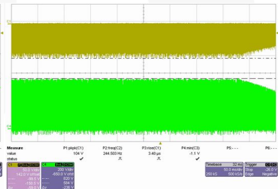
Figure 25. 264 V / 50 Hz at Maximum Load (Turns Off), Ch1: V_{DS}(\text{MOSFET}) , Ch4: V_{AK}(\text{RECTIFIER})
