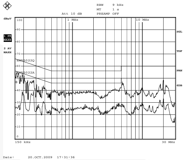
Figure 26. Conduction-Line & Neutral at 115V AC
