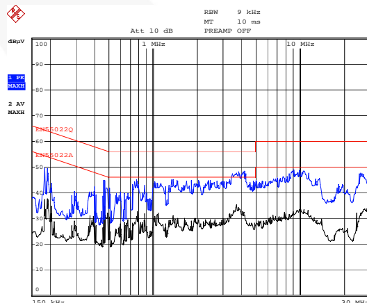
Figure 19. L: 230 / 50Hz
