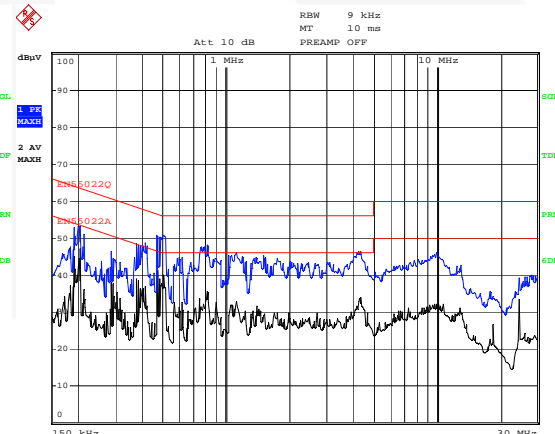
Figure 18. N: 115 / 60Hz
