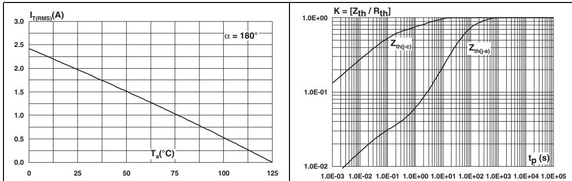
Figure 3. On-state rms current versus ambient temperature (free air convection) Figure 4. Relative variation of thermal impedance versus pulse duration
