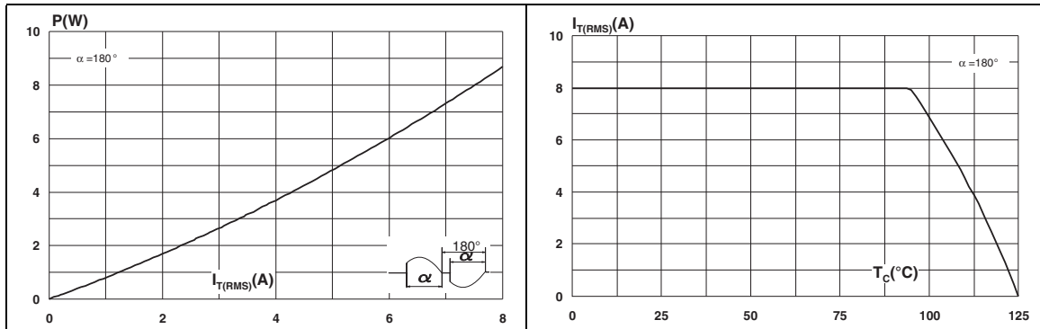
Figure 1. Maximum power dissipation versus rms on-state current Figure 2. On-state rms current versus case temperature
